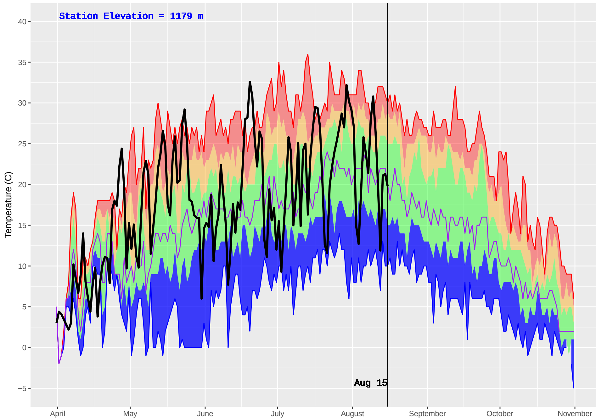
HOLMES (201) : Historical (1987–2016) and Current (2018) Daily Temperature
