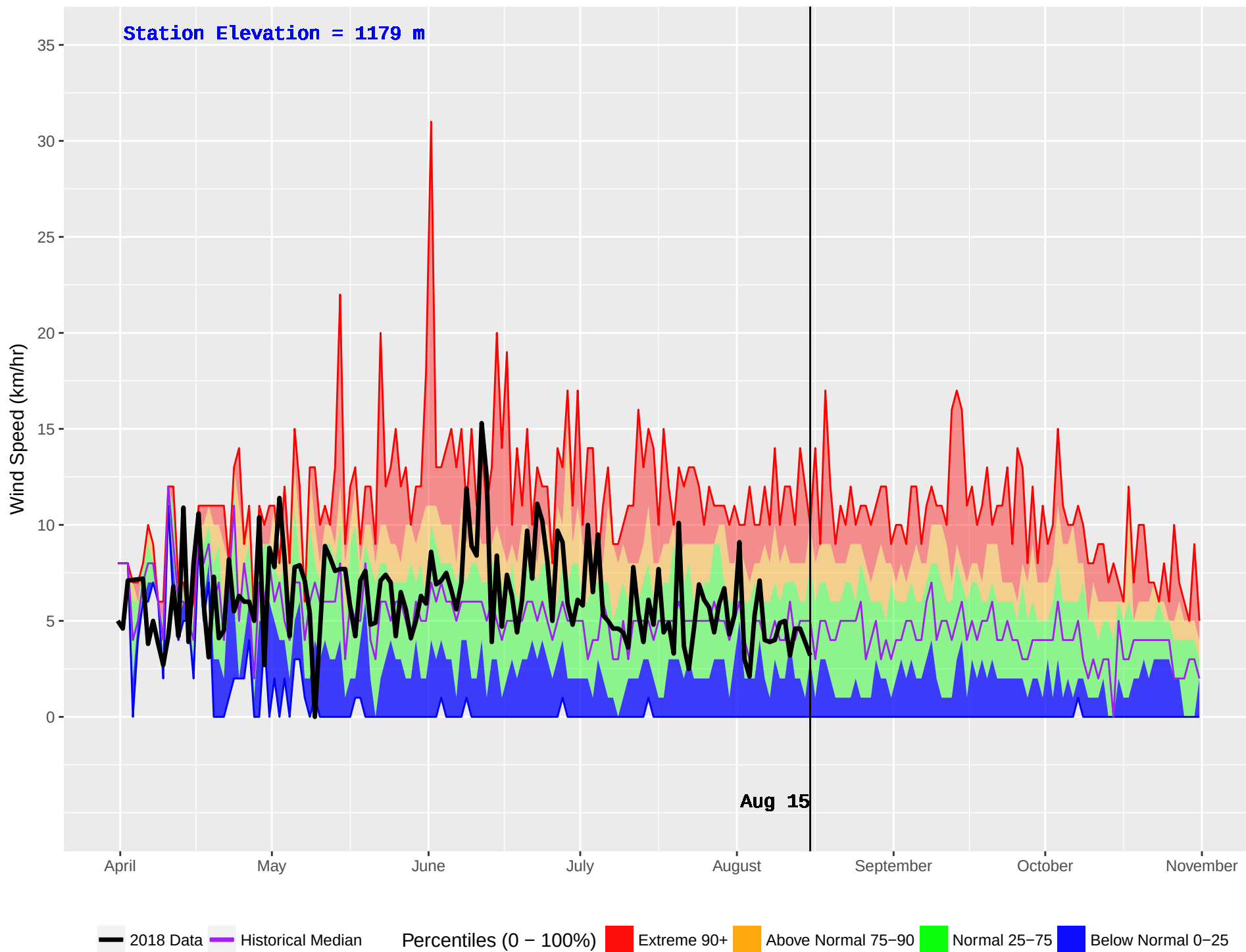
HOLMES (201) : Historical (1987–2016) and Current (2018) Daily Wind Speed
