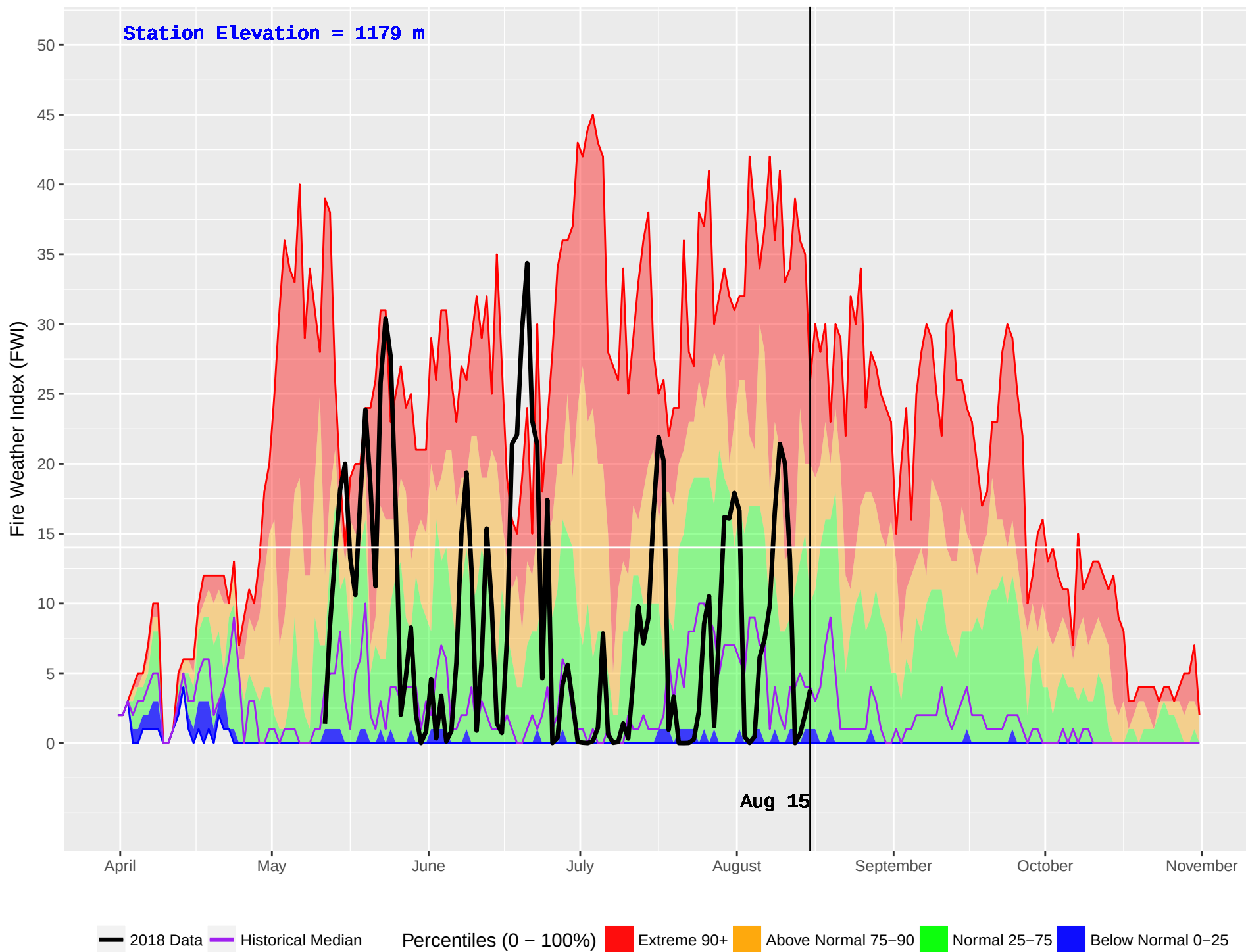
HOLMES (201) : Historical (1987–2016) and Current (2018) Daily Fire Weather Index (FWI)
