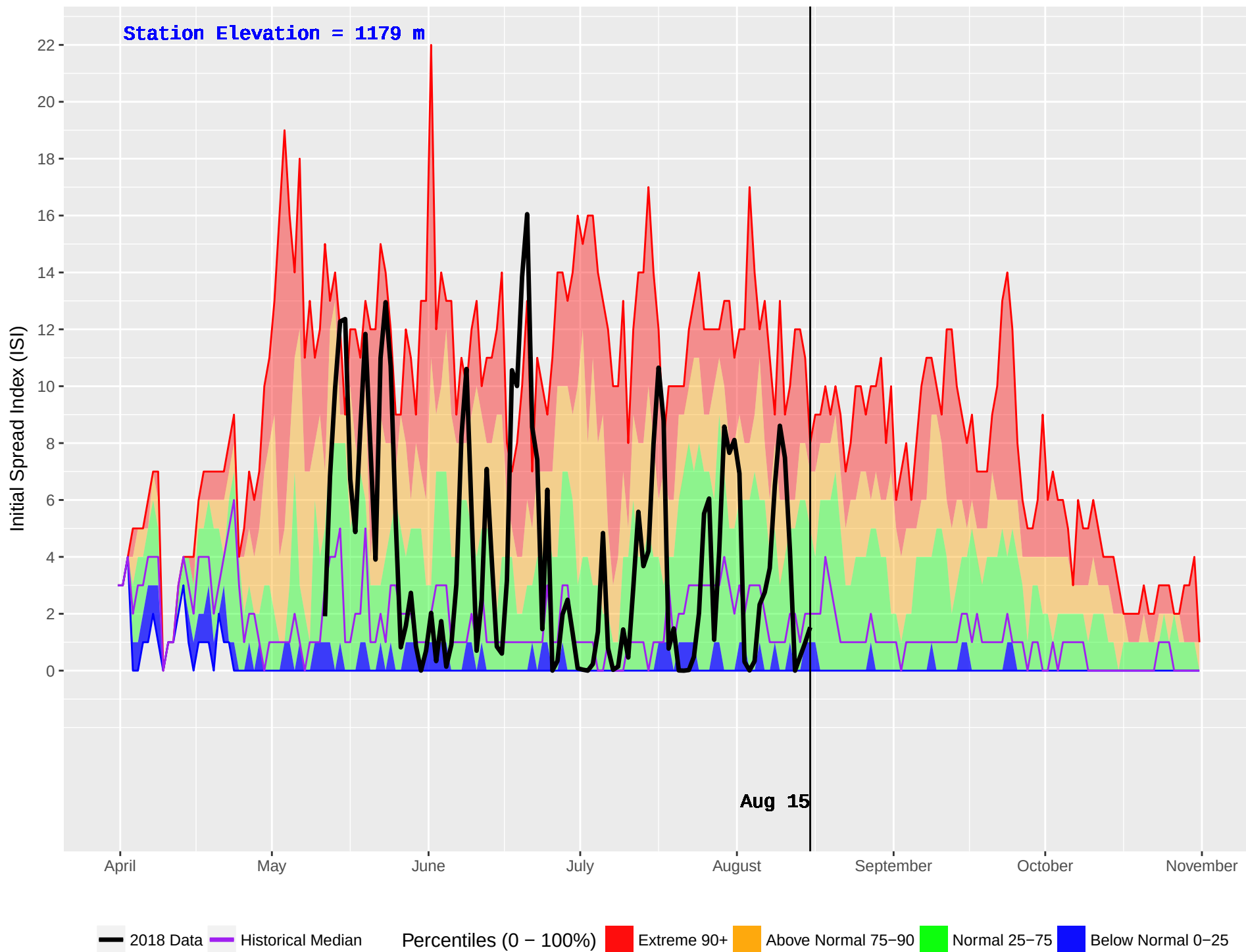
HOLMES (201) : Historical (1987–2016) and Current (2018) Daily Initial Spread Index (ISI)
