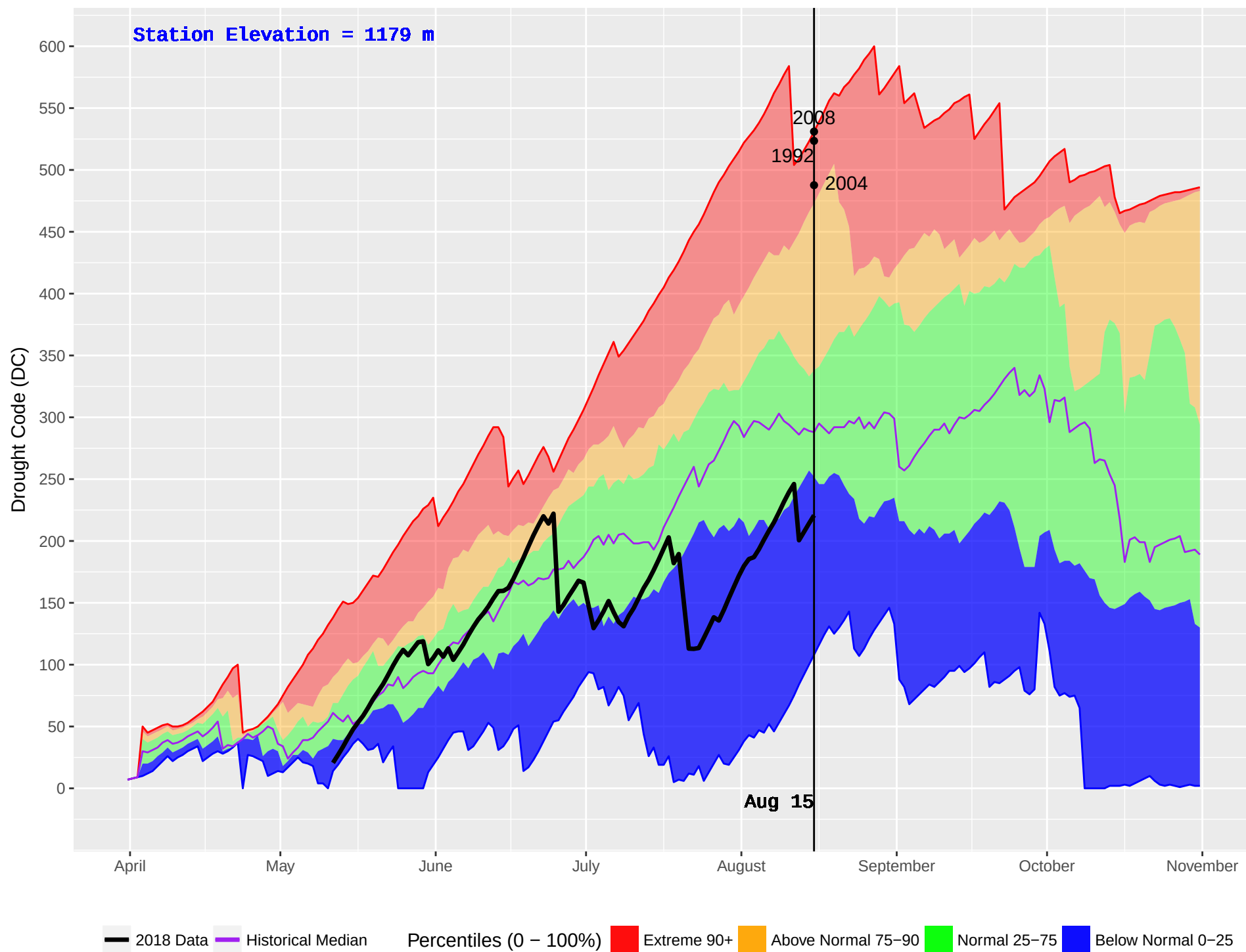
HOLMES (201) : Historical (1987–2016) and Current (2018) Daily Drought Code (DC)
